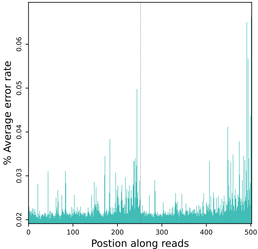
Error rate distribution along reads (R10213)
